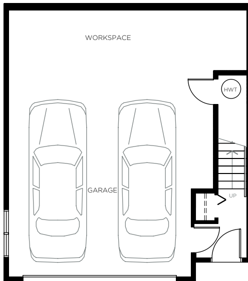
LOWER LEVEL
