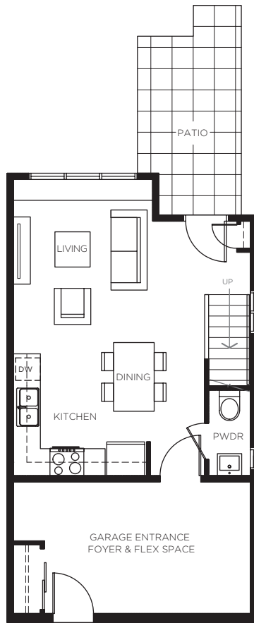
LOWER LEVEL
